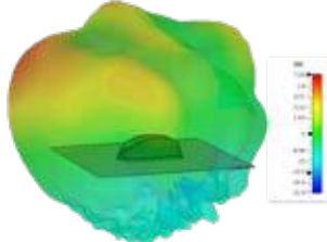
3D Plot Element 2 Side (2600 MHz)
