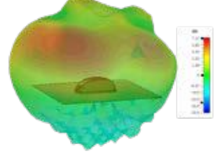
3D Plot Element 1 Side (2600 MHz)
