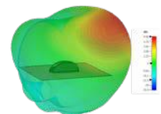
3D Plot Element 4 Side (1800 MHz)
