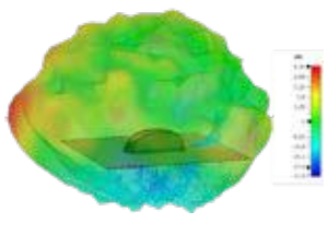
3D Plot Element 1 Side (5400 MHz)
