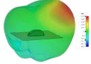
3D Plot Element 4 Side (850 MHz)
