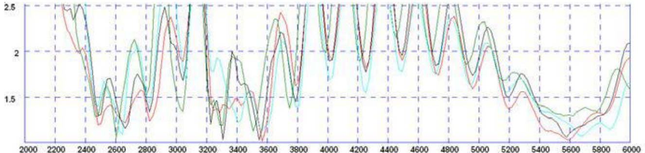
Typical VSWR*
